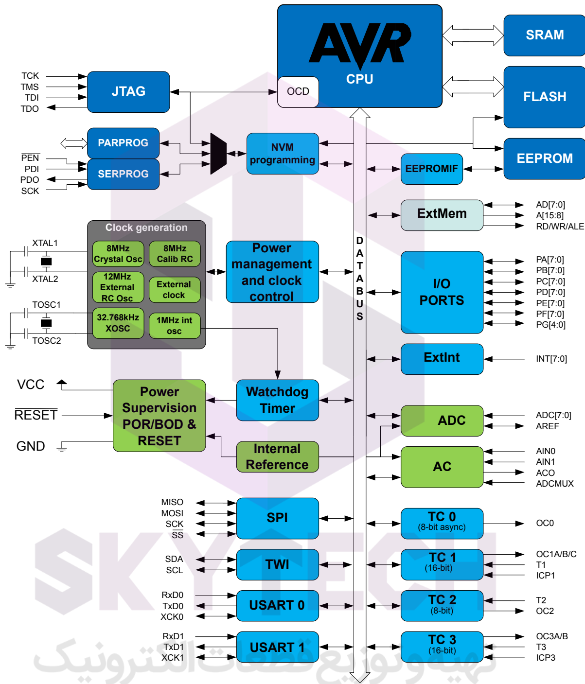
Figure 4-1 Block Diagram
